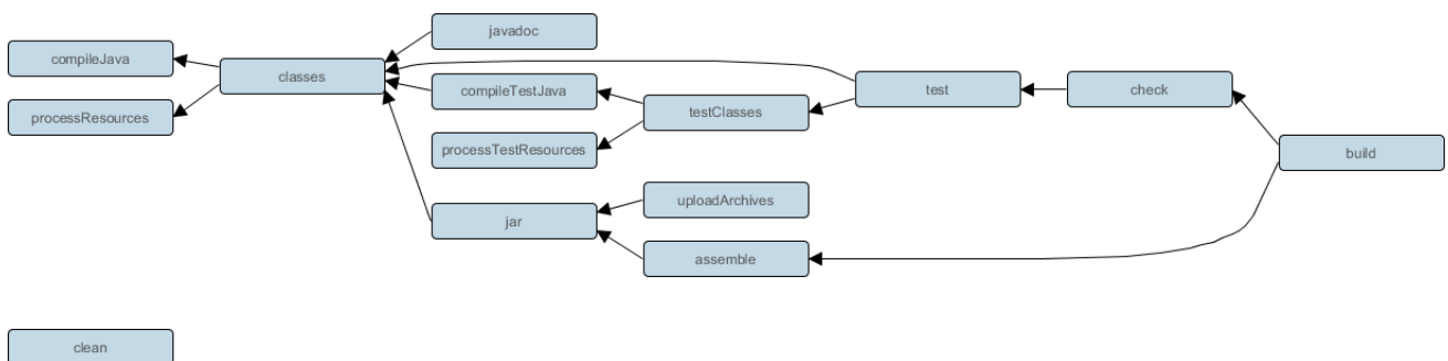
Figure 31. Java plugin - tasks
