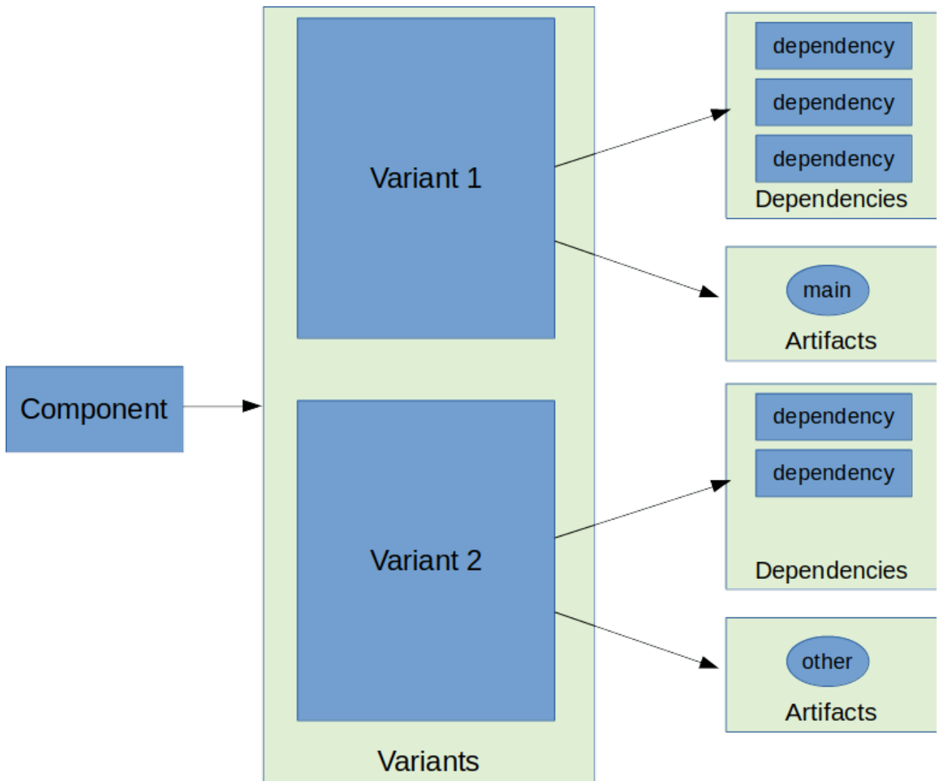
Figure 20. The Gradle component model
