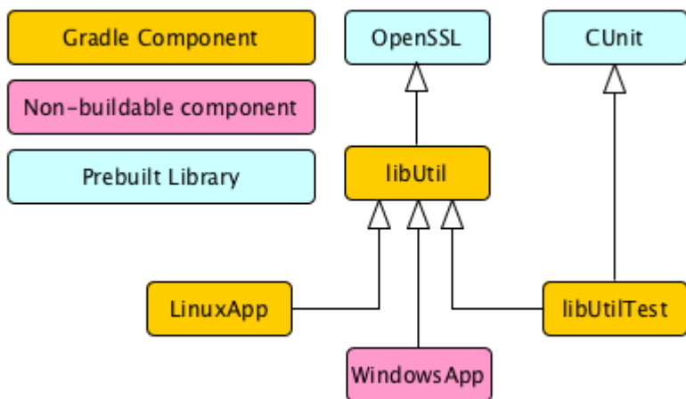
Figure 26. Dependent Components Example
