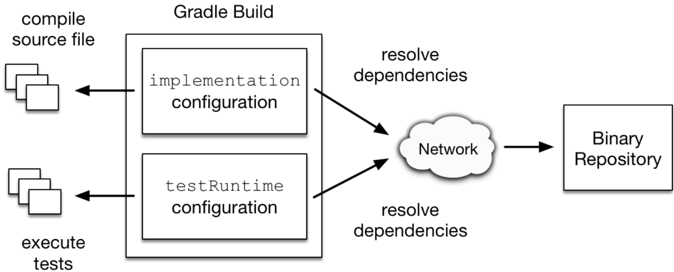
Figure 14. Configurations use declared dependencies for specific purposes
