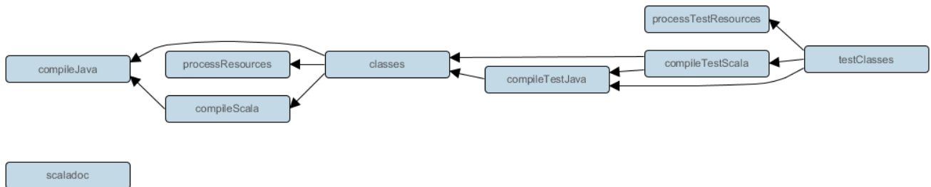
Figure 34. Scala plugin - tasks
