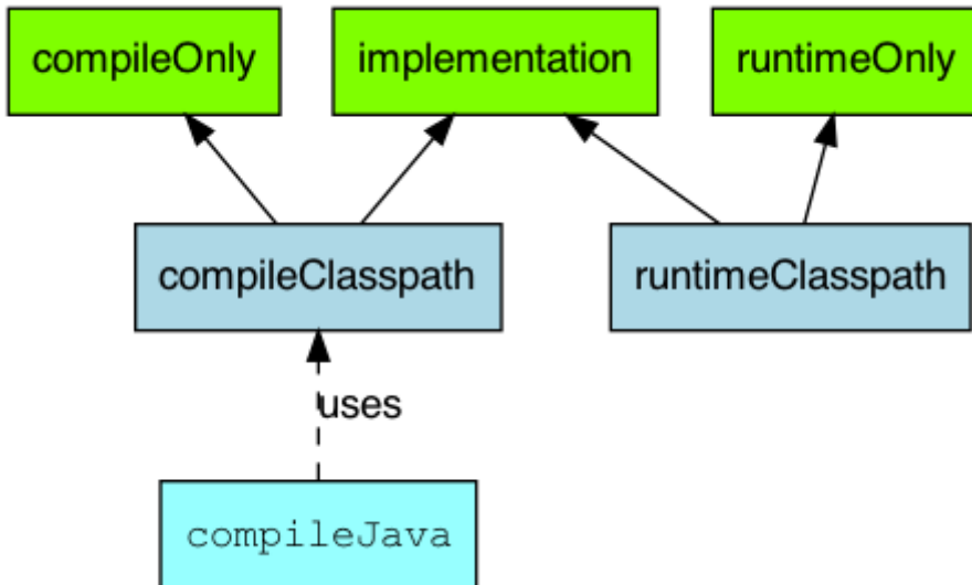
Figure 32. Java plugin - main source set dependency configurations
