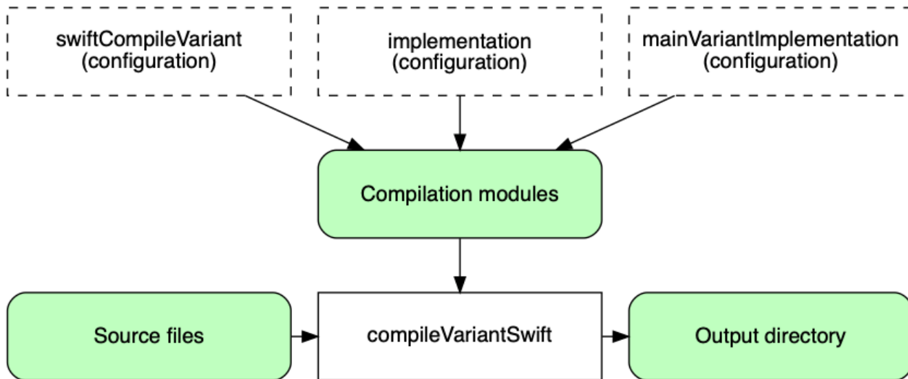
Figure 25. Sources and Swift compilation
