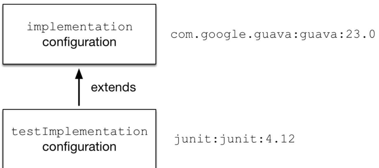
Figure 15. Configuration inheritance provided by the Java plugin
