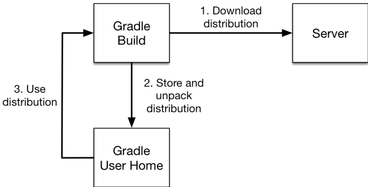
Figure 29. The Wrapper workflow
