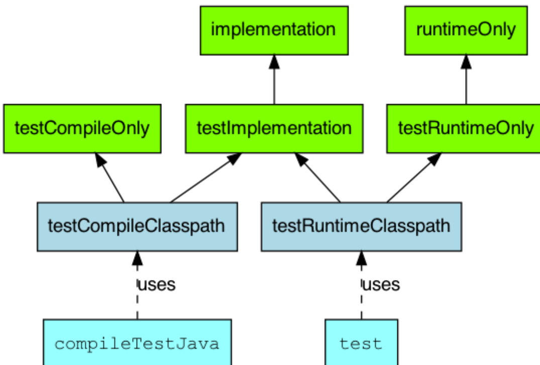
Figure 33. Java plugin - test source set dependency configurations
