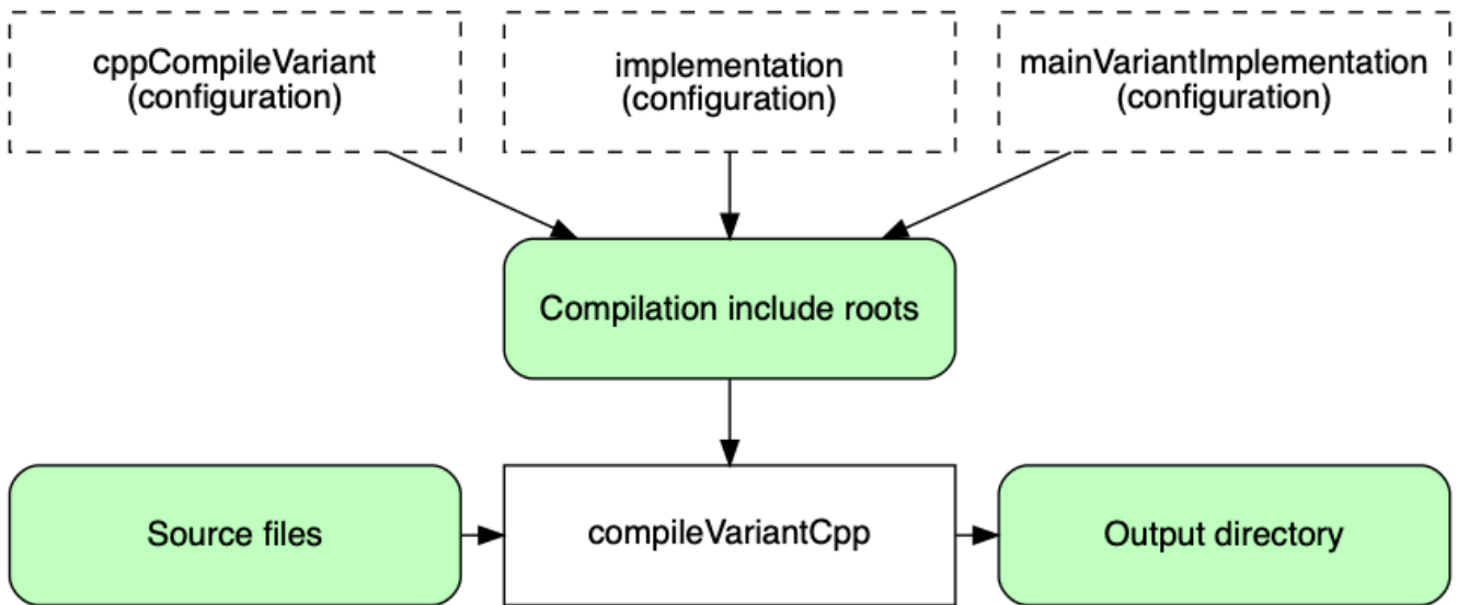
Figure 24. Sources and C++ compilation
