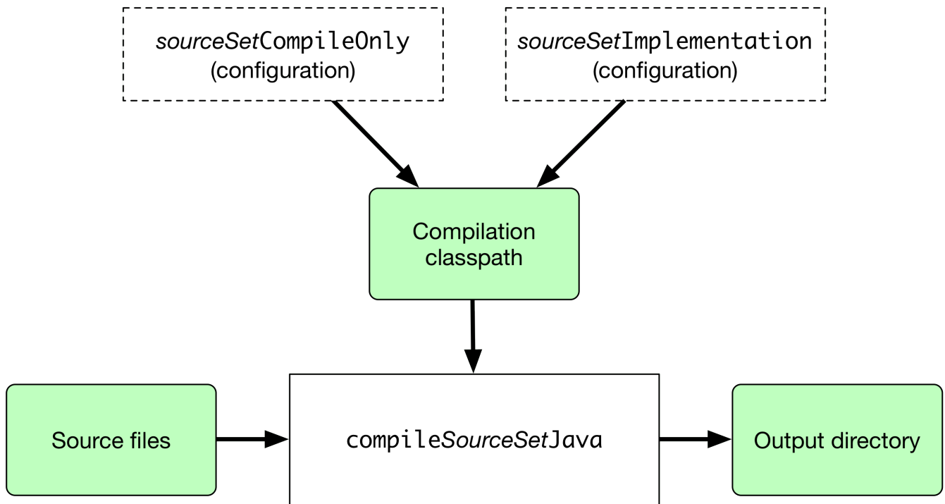
Figure 22. Source sets and Java compilation
