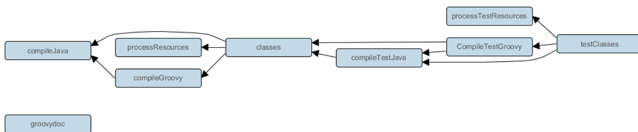
Figure 30. Groovy plugin - tasks
